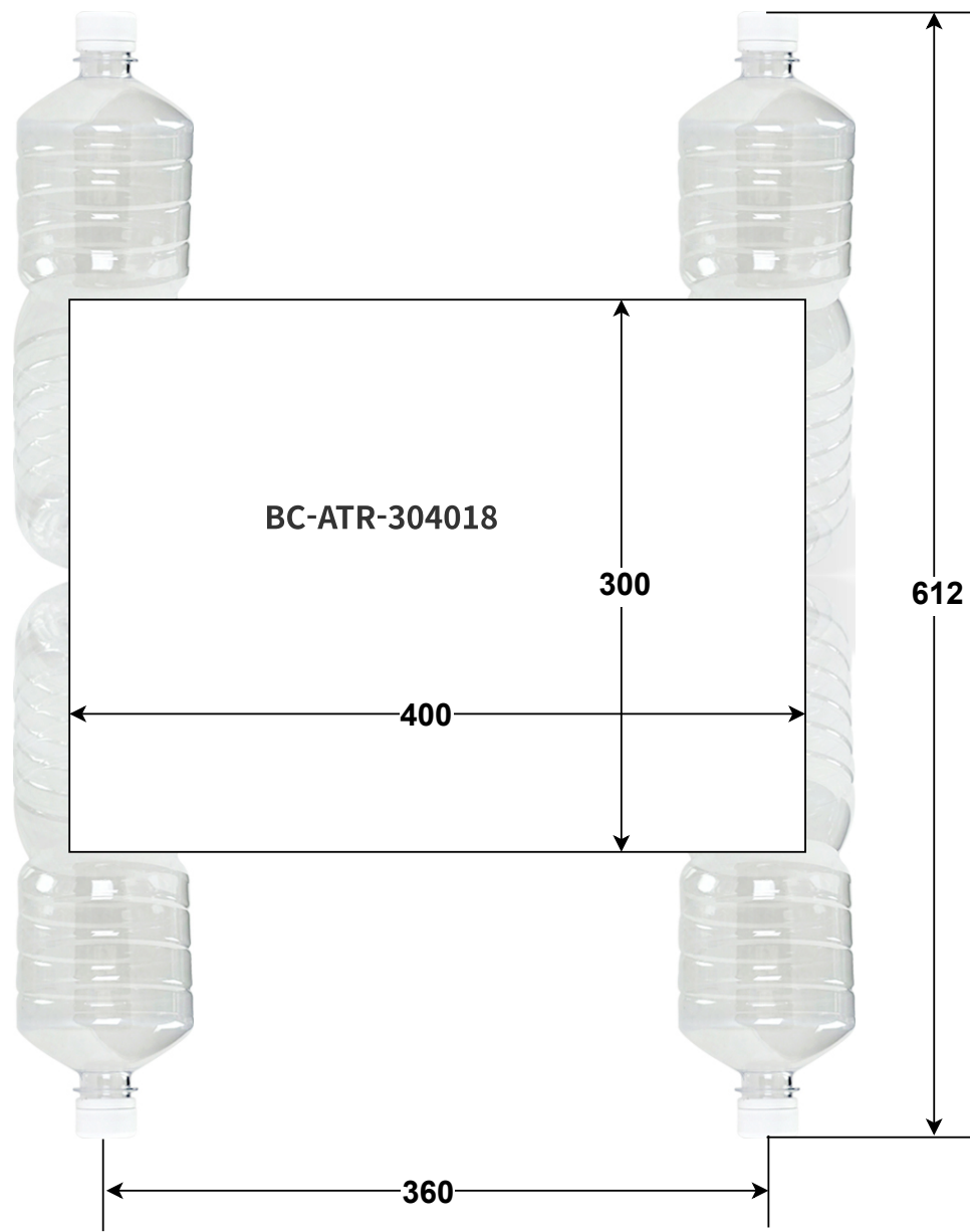
TEST USV1 FRAME STRUCTURE DIAGRAM r0.1
